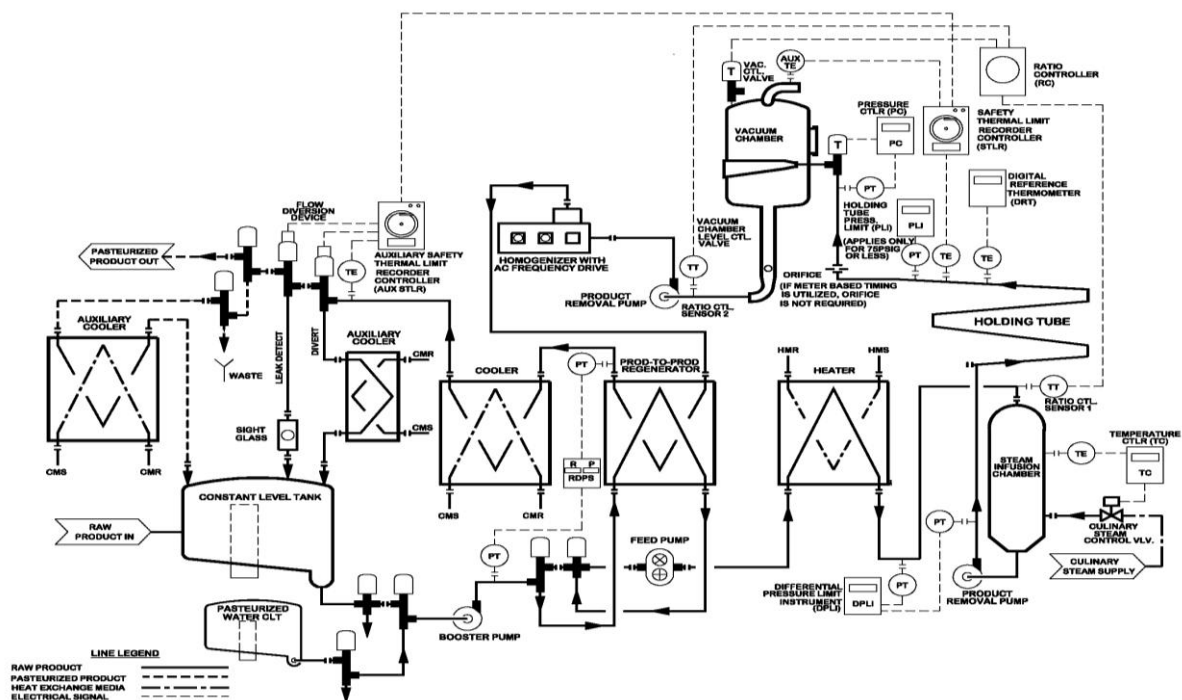
Figure 42. HHST Pasteurizer Utilizing Direct Culinary Steam Infusion and Vacuum Flash Cooling with a Homogenizer Located Downstream
